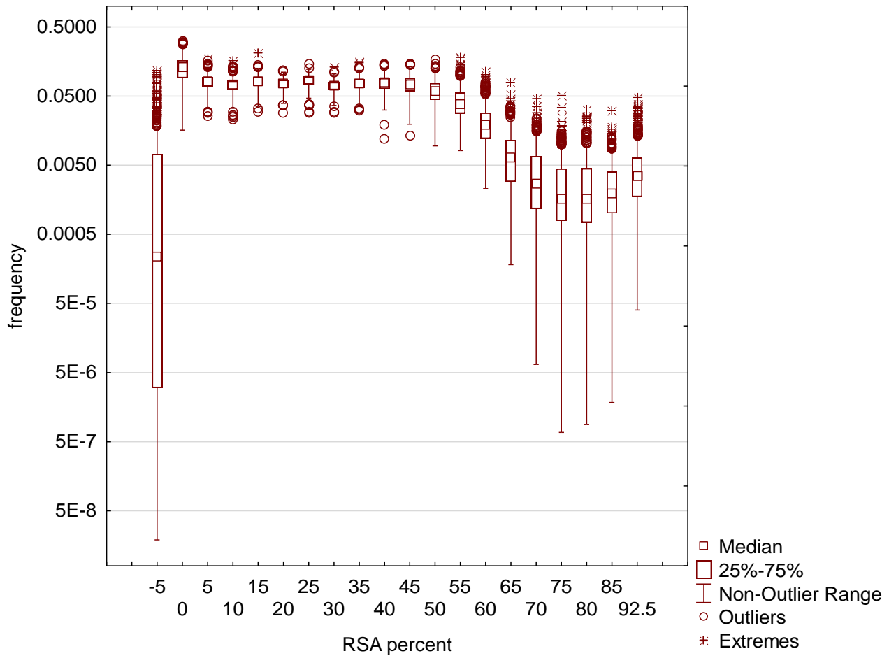
Fig S2.2 Frequencies of RSA percent categories in data under analysis, log scale.
